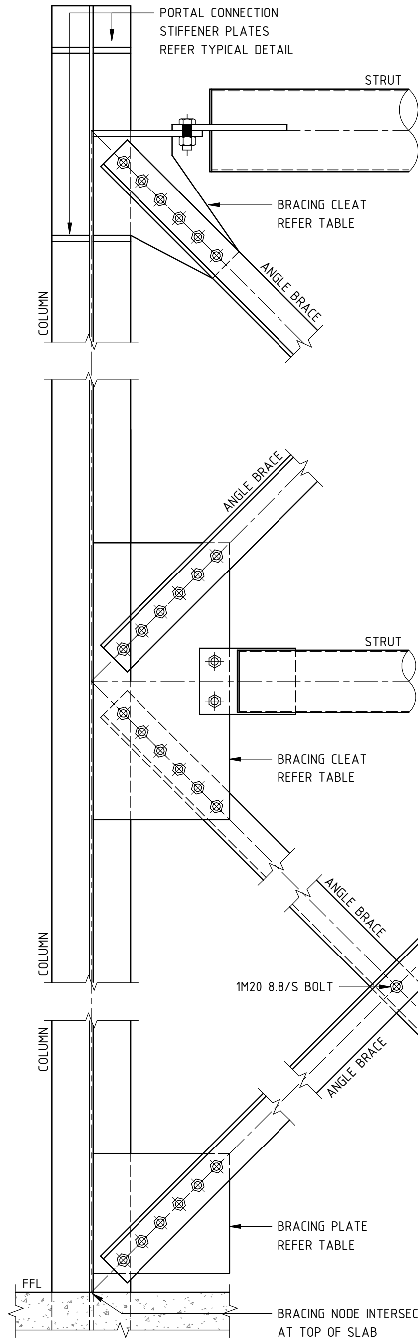
TYPICAL WALL BRACING CONFIGURATIONS COLUMN FLANGE REMOVED FOR CLARITY
