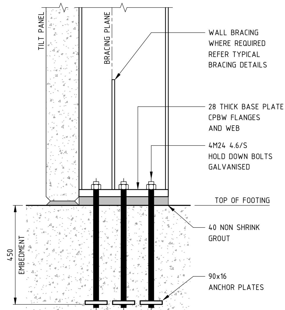
TYPICAL END WALL COLUMN BASE PLATE DETAIL
