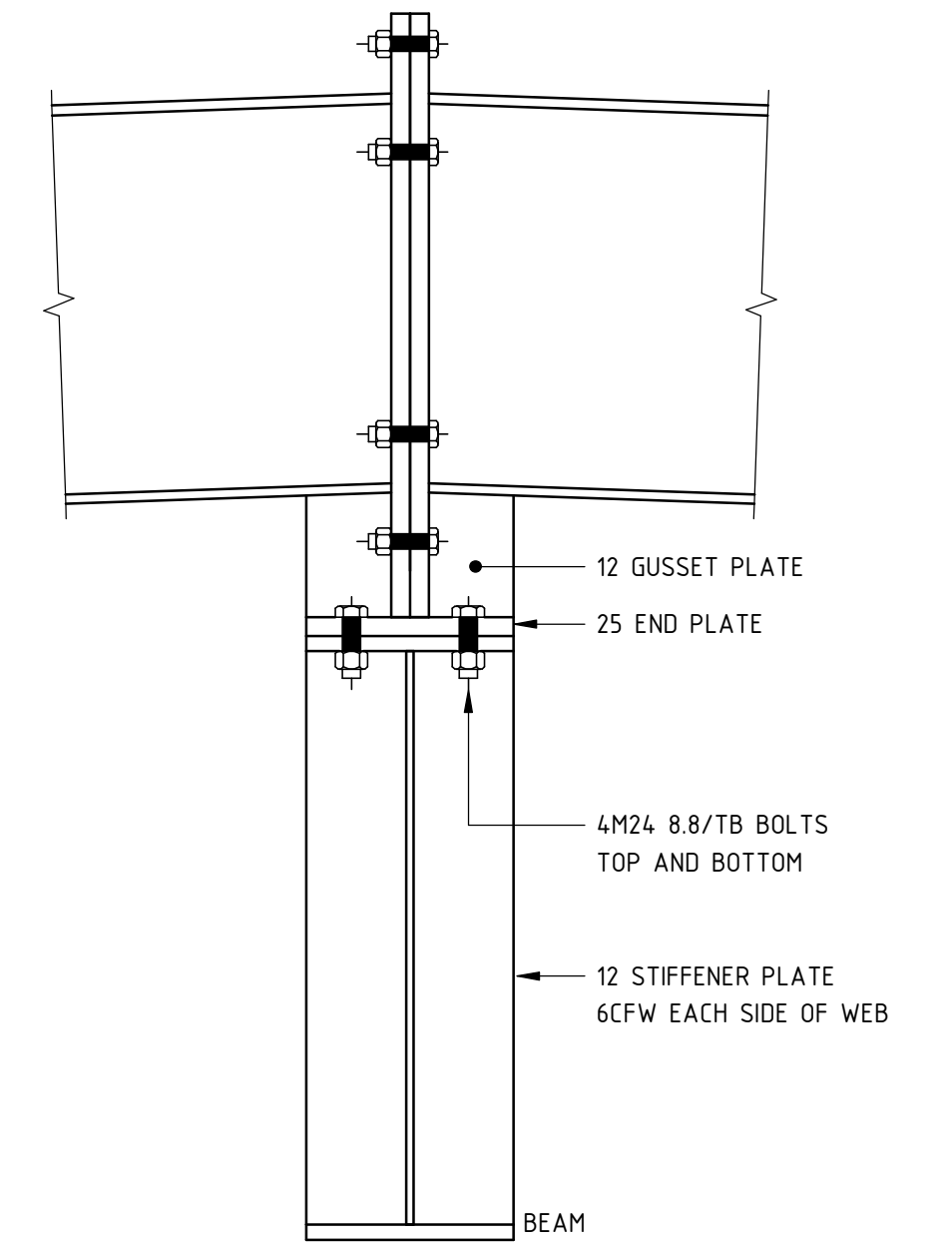
TYPICAL TRANSFER BEAM SUPPORT CONNECTION DETAIL
