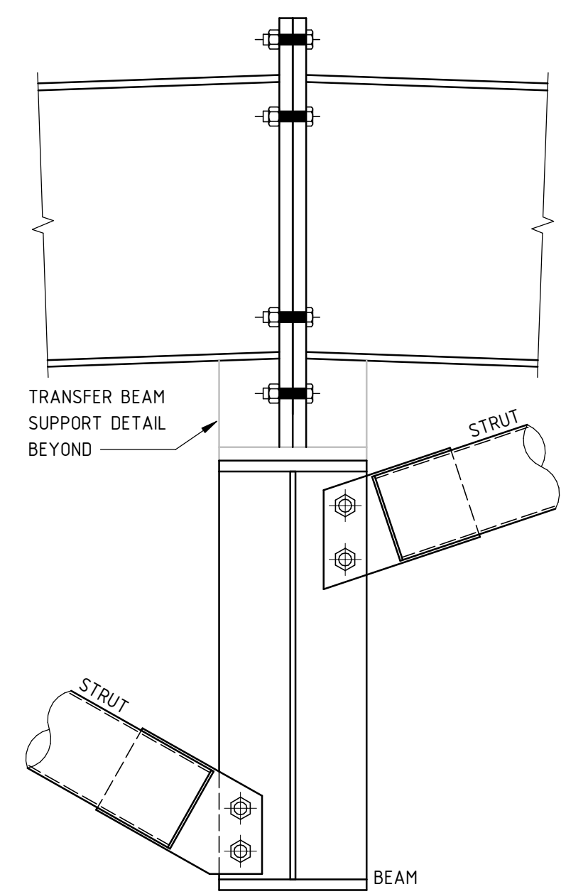
TYPICAL TRANSFER BEAM SUPPORT CONNECTION DETAIL
