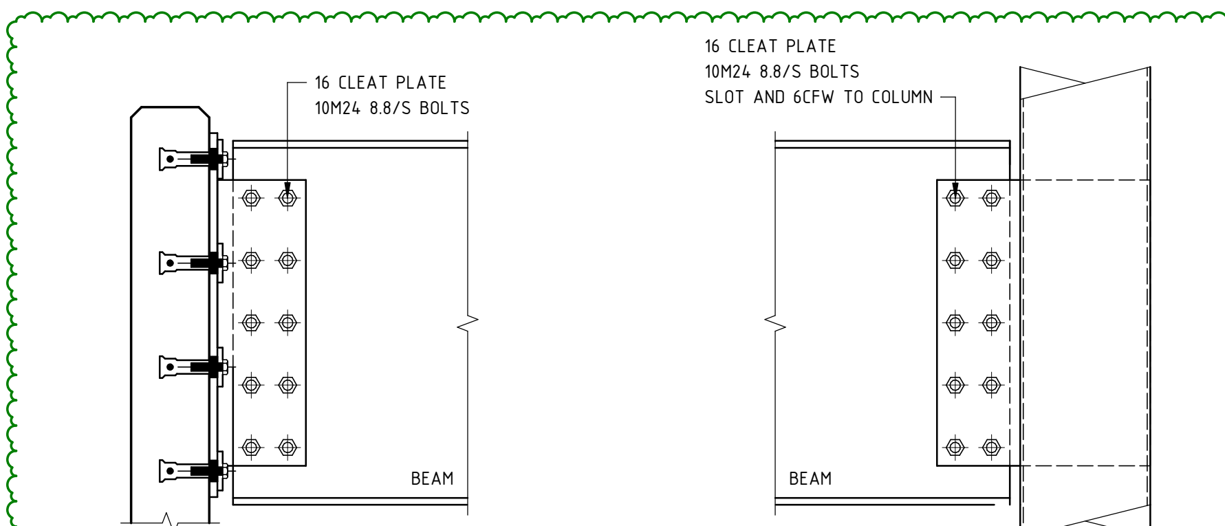
TYPICAL TRANSFER BEAM TO PRECAST CONNECTION DETAIL
