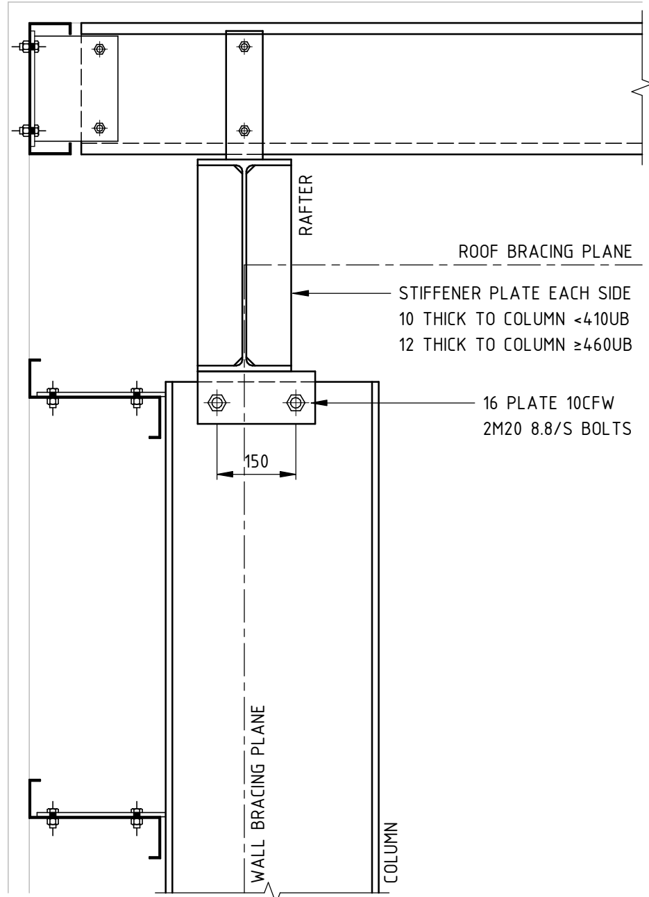
TYPICAL END WALL COLUMN TO RAFTER DETAIL
