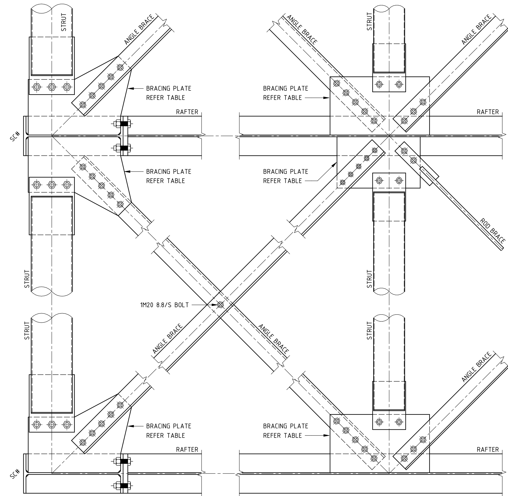
TYPICAL ROOF BRACING CONFIGURATIONS RAFTER TOP FLANGE REMOVED FOR CLARITY
