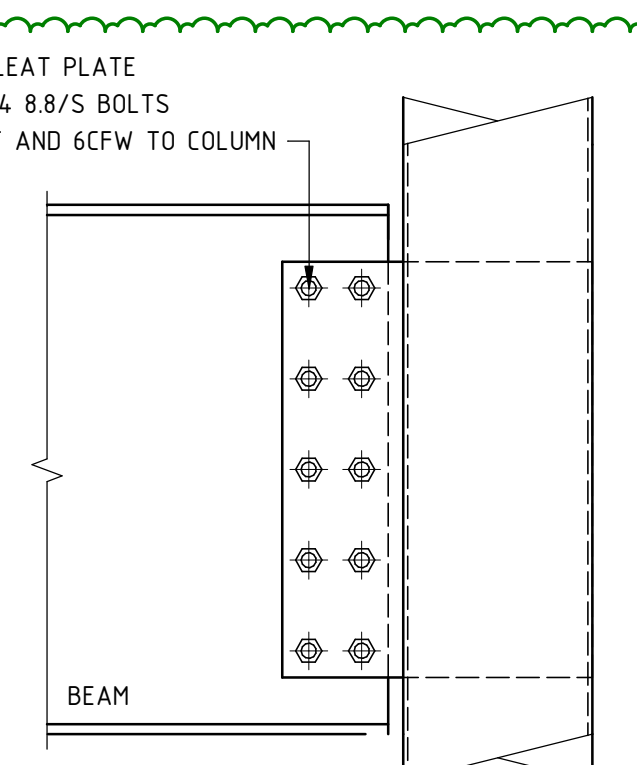
TYPICAL TRANSFER BEAM TO COLUMN CONNECTION DETAIL
