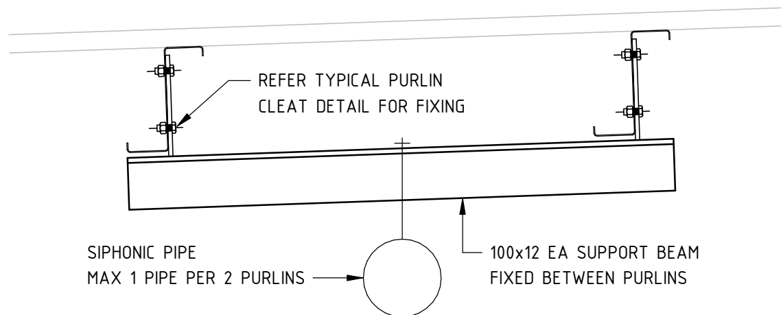
TYPICAL SIPHONIC PIPE SUPPORT FRAME DETAIL
