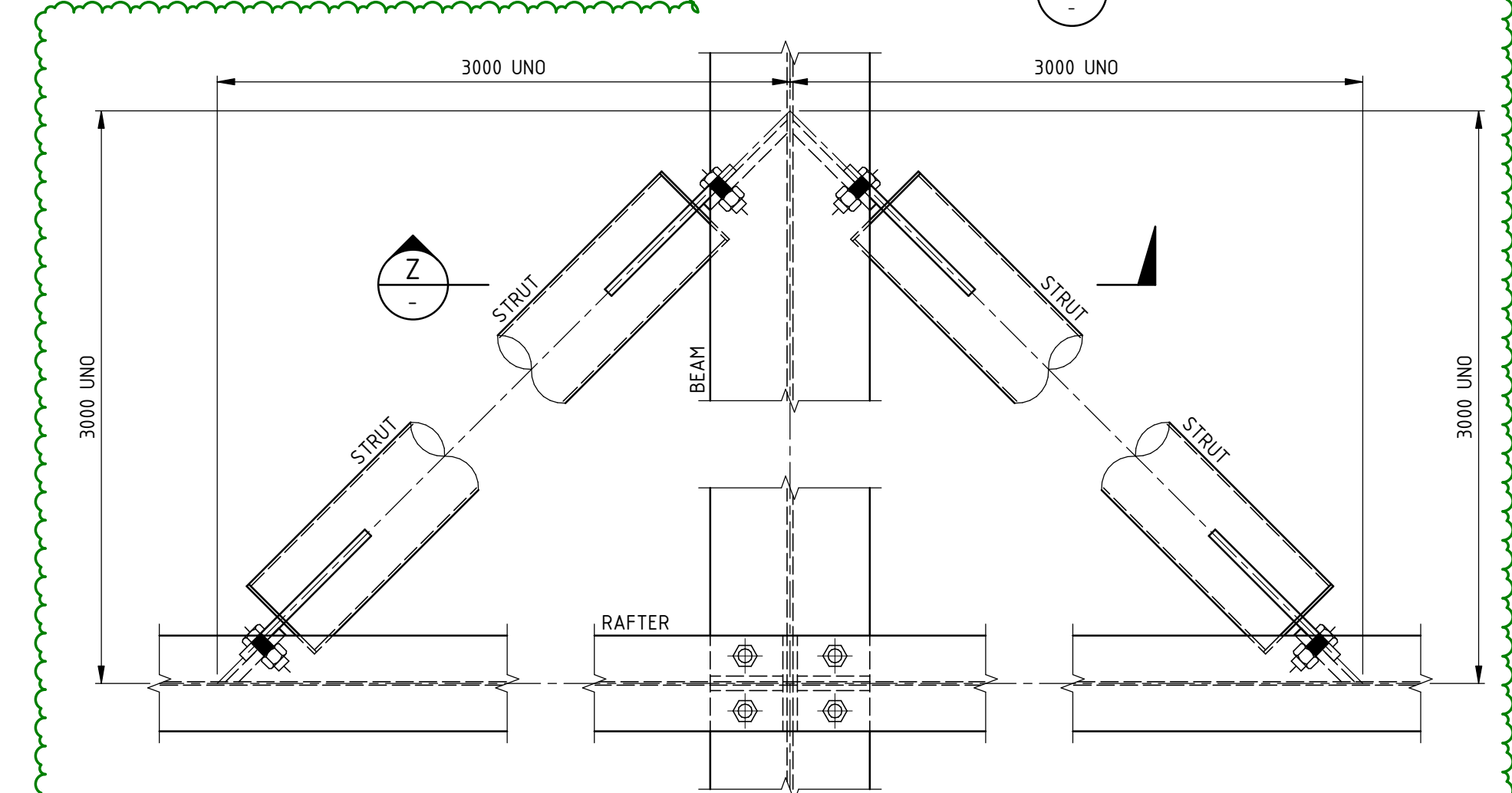
TYPICAL TRANSFER BEAM BRACING DETAIL
